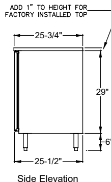
Side Elevation
